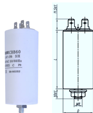
FM faston 6,3mm +(matica) vijak M8
