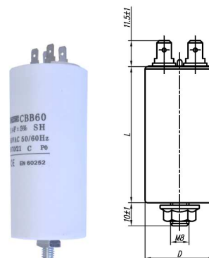
FM faston 6,3mm +(matica) vijak M8
