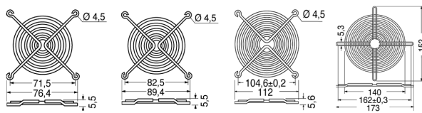
80x80mm 92x92mm 120x120mm 172x150mm
